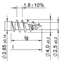
cut
